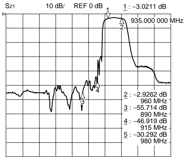
Filter 1 (Passband : 935 MHz to 960 MHz)
