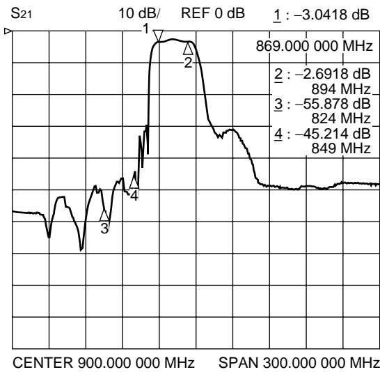
Filter 1 (Passband : 869 MHz to 894 MHz)
