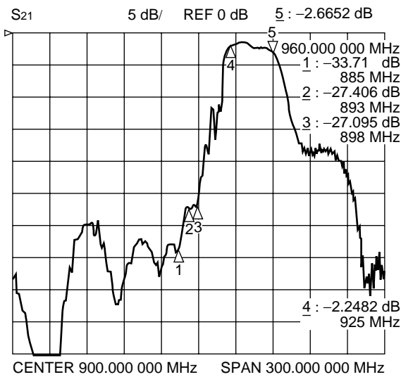
Filter 2 (Passband : 925 MHz to 960 MHz)
