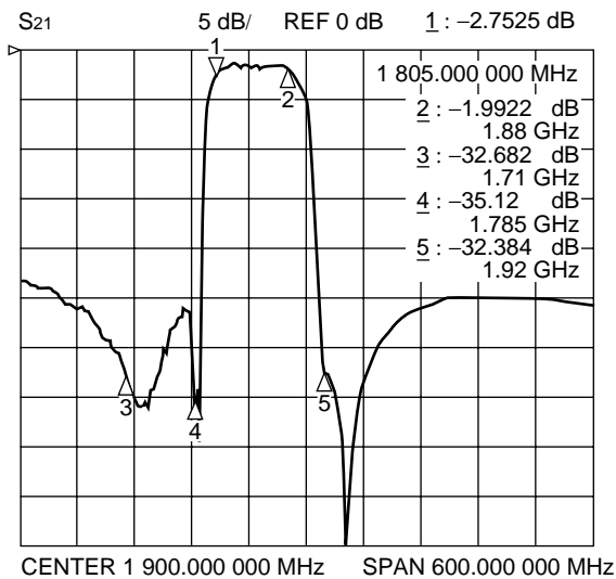
Filter 2 (Passband : 1805 MHz to 1880 MHz)
