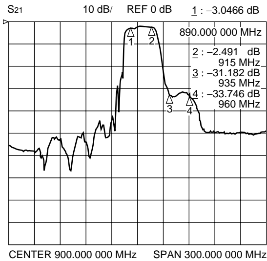
Filter 1 (Passband : 890 MHz to 915 MHz)
