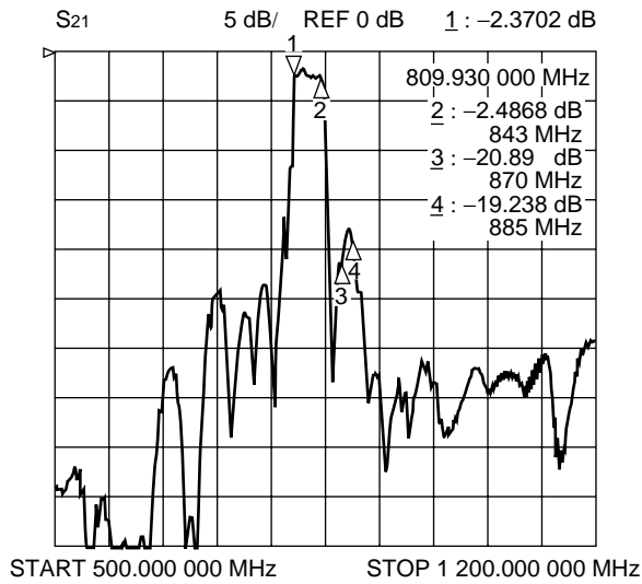
Filter 1 (Passband : 810 MHz to 843 MHz)
