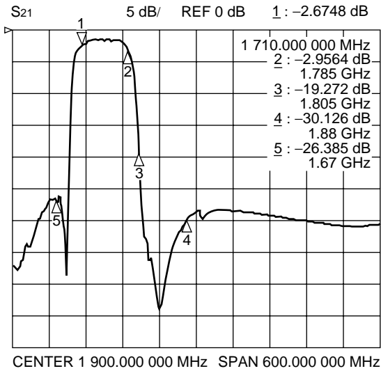
Filter 2 (Passband : 1710 MHz to 1785 MHz)
