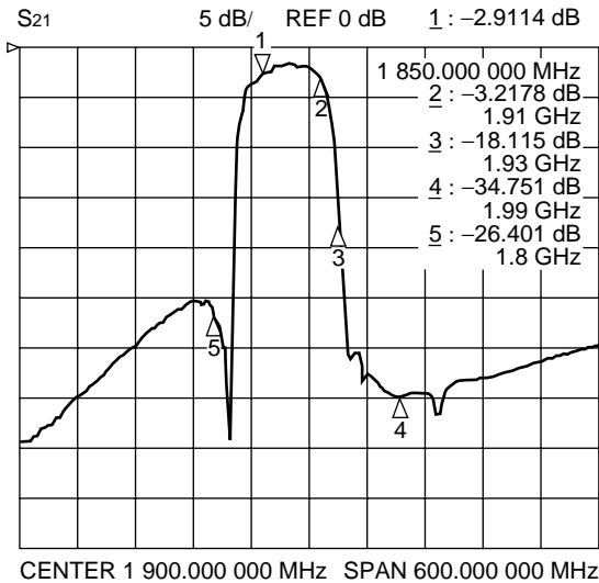
Filter 2 (Passband : 1850 MHz to 1910 MHz)
