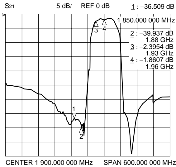
Filter 1 (Passband : 1930 MHz to 1960 MHz)
