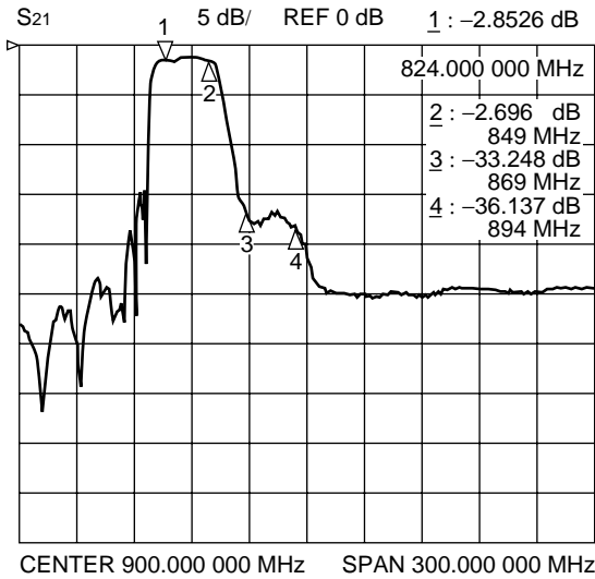
Filter 1 (Passband : 824 MHz to 849 MHz)
