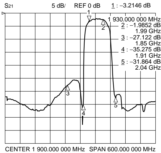
Filter 2 (Passband : 1930 MHz to 1960 MHz)
