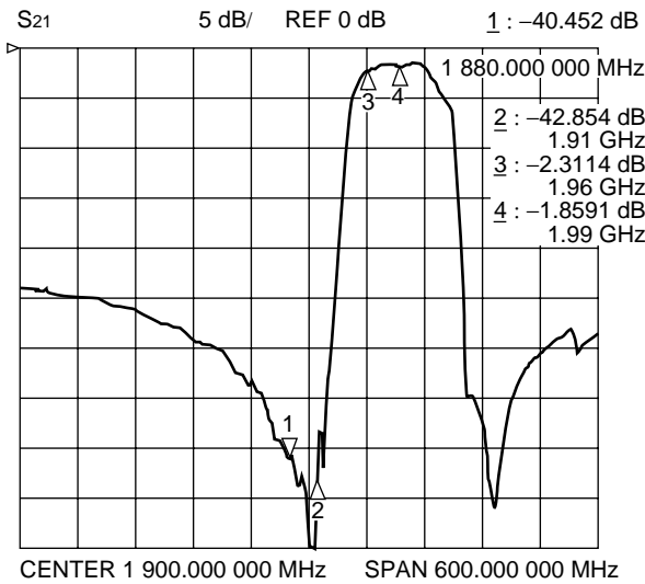
Filter 2 (Passband : 1960 MHz to 1990 MHz)
