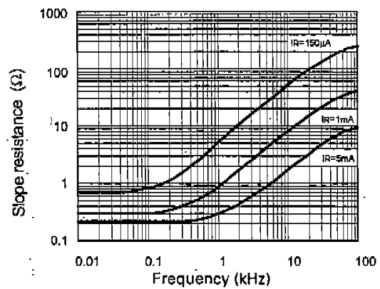
Slope Resistance v Frequency
