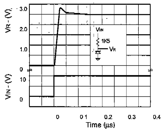
Transient Response ( I_R = 5\text{mA} )
