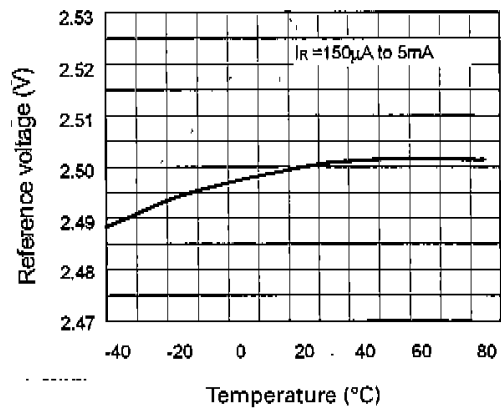
Temperature Drift
