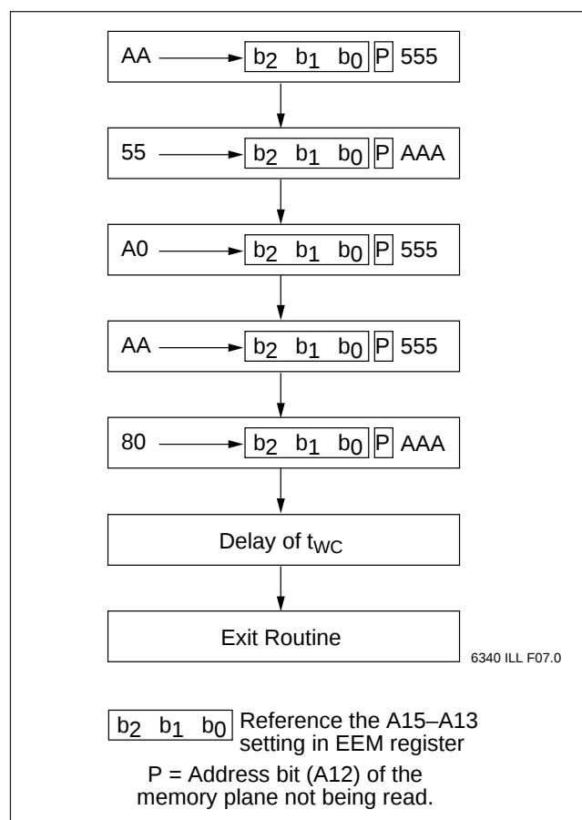
Figure 4. Sequence to Deactivate Software Data Protection
