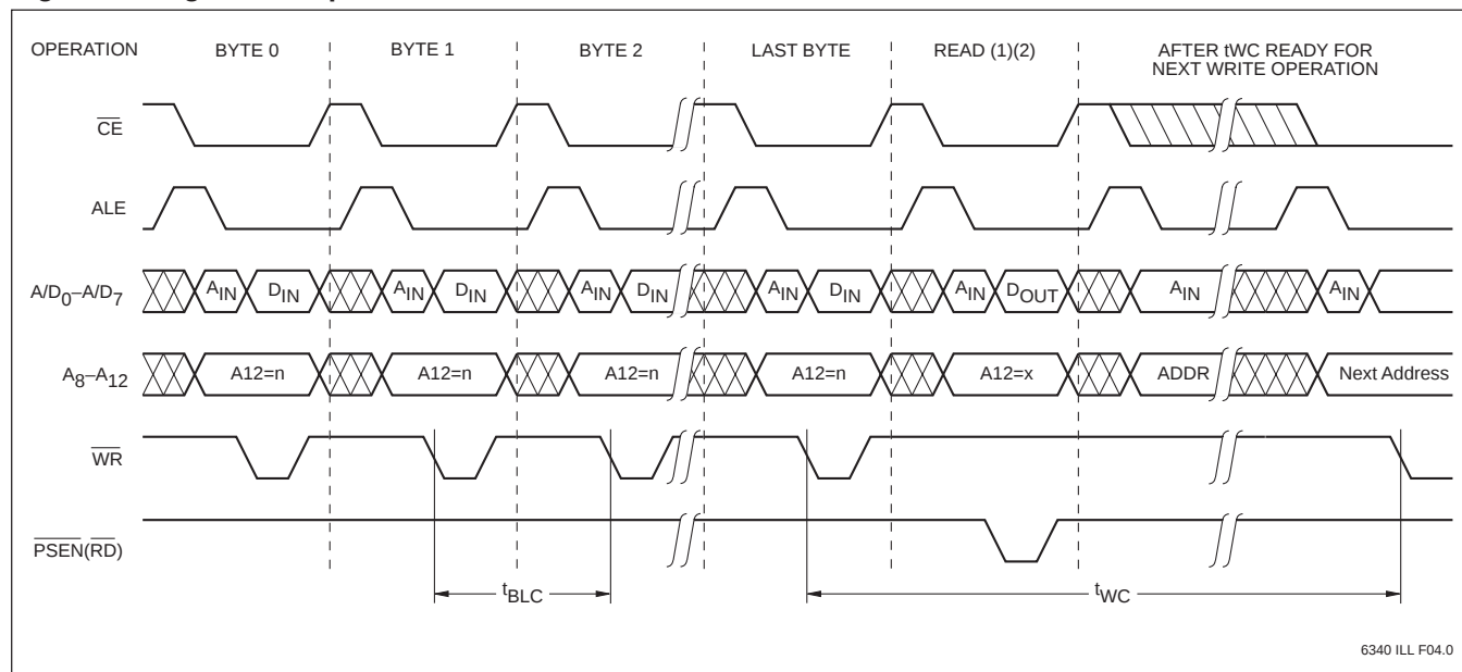
Figure 1. Page Write Operation
