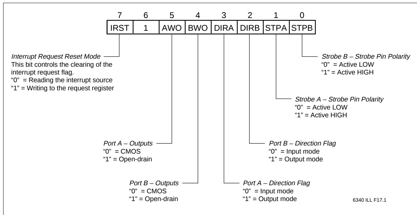
Figure 12. Configuration Register
