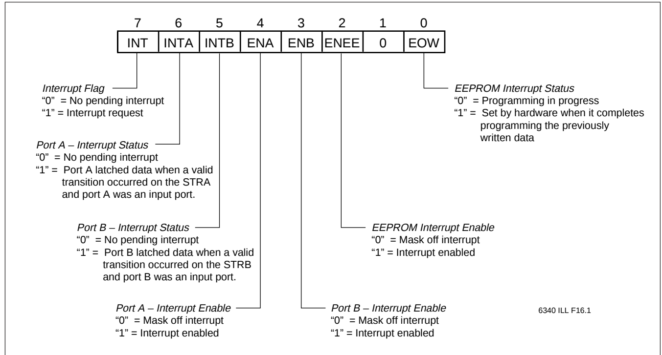
Figure 11. Interrupt Status Register
