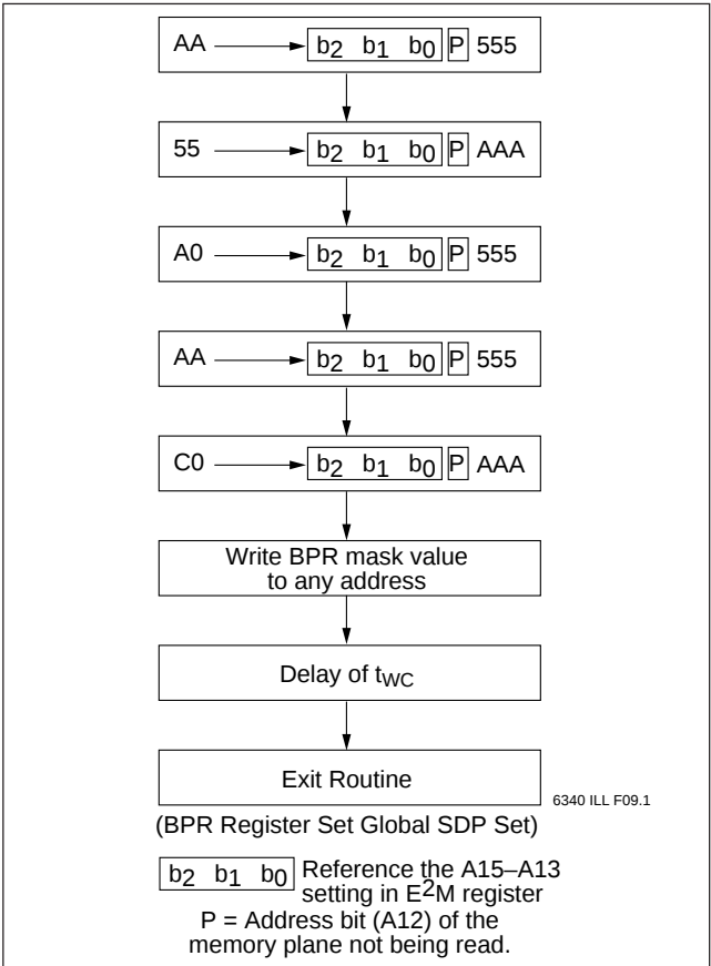
Figure 6. Setting BPR Command Sequence
