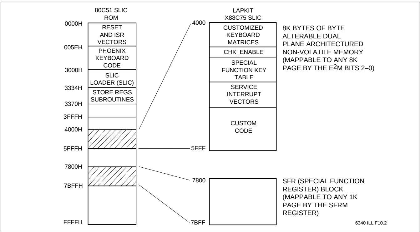
Figure 7. Microcontroller Map
