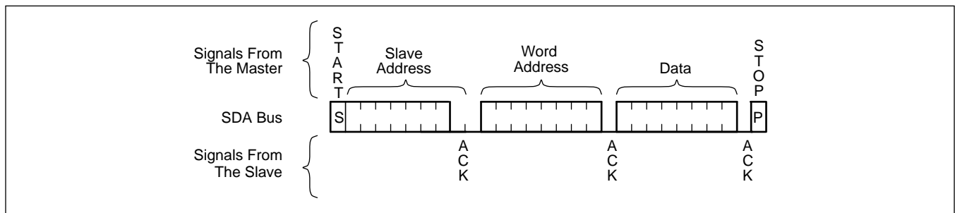
Figure 5. Byte Write Sequence
