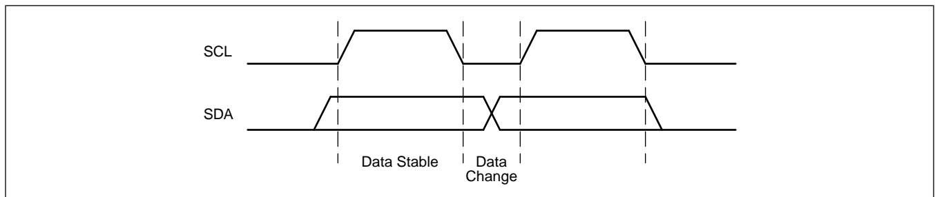
Figure 1. Data Validity
