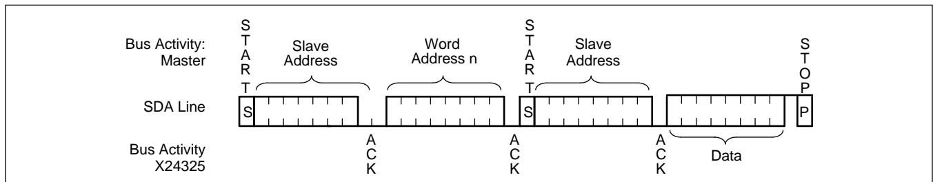
Figure 8. Random Read
