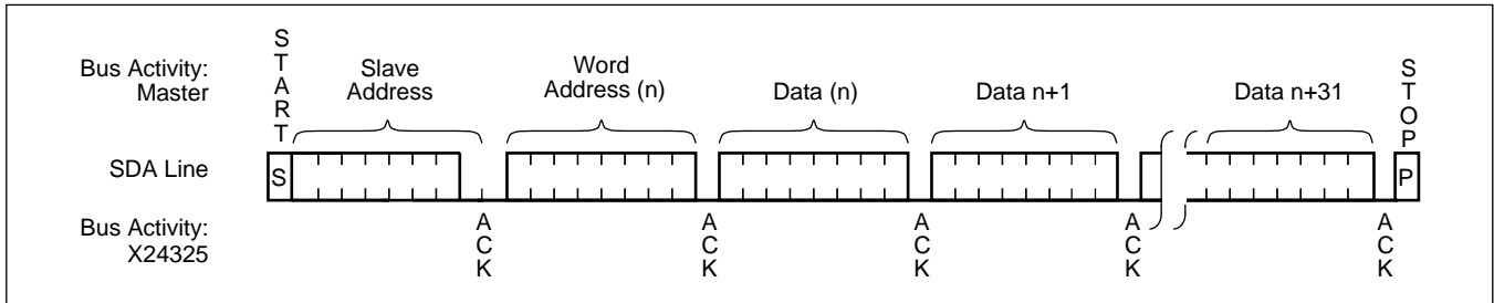
Figure 6. Page Write Sequence
