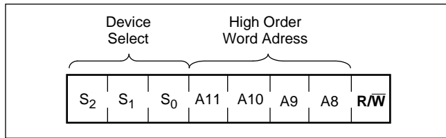
Figure 4. Slave Address
