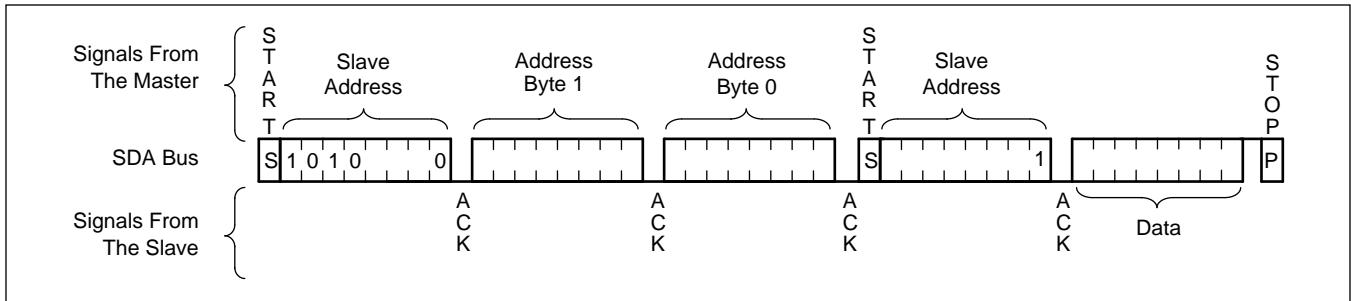
Figure 9. Random Read Sequence
