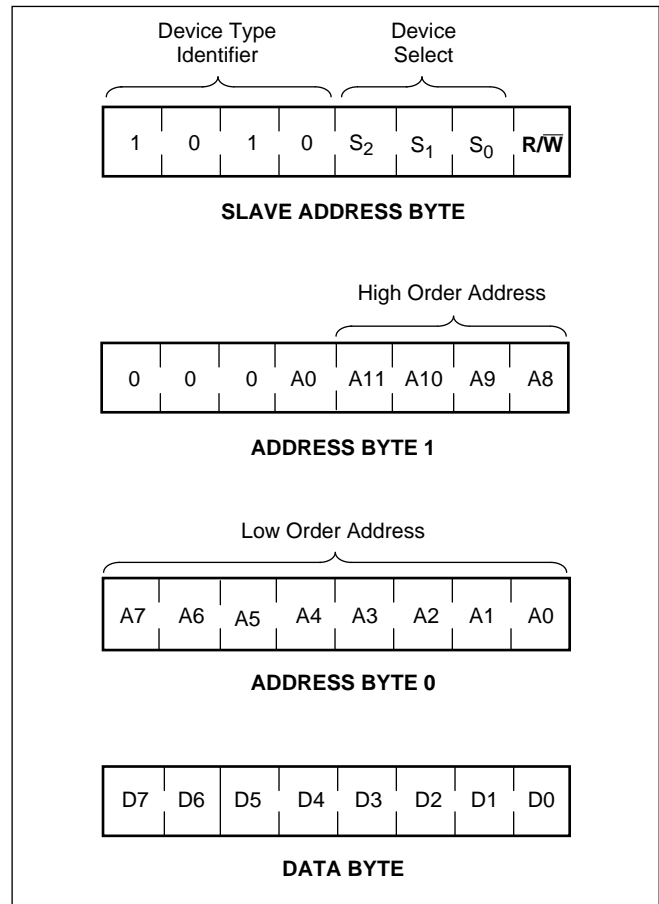
Figure 4. Device Addressing
