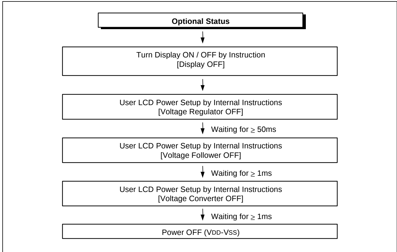
Figure 27. Power OFF
