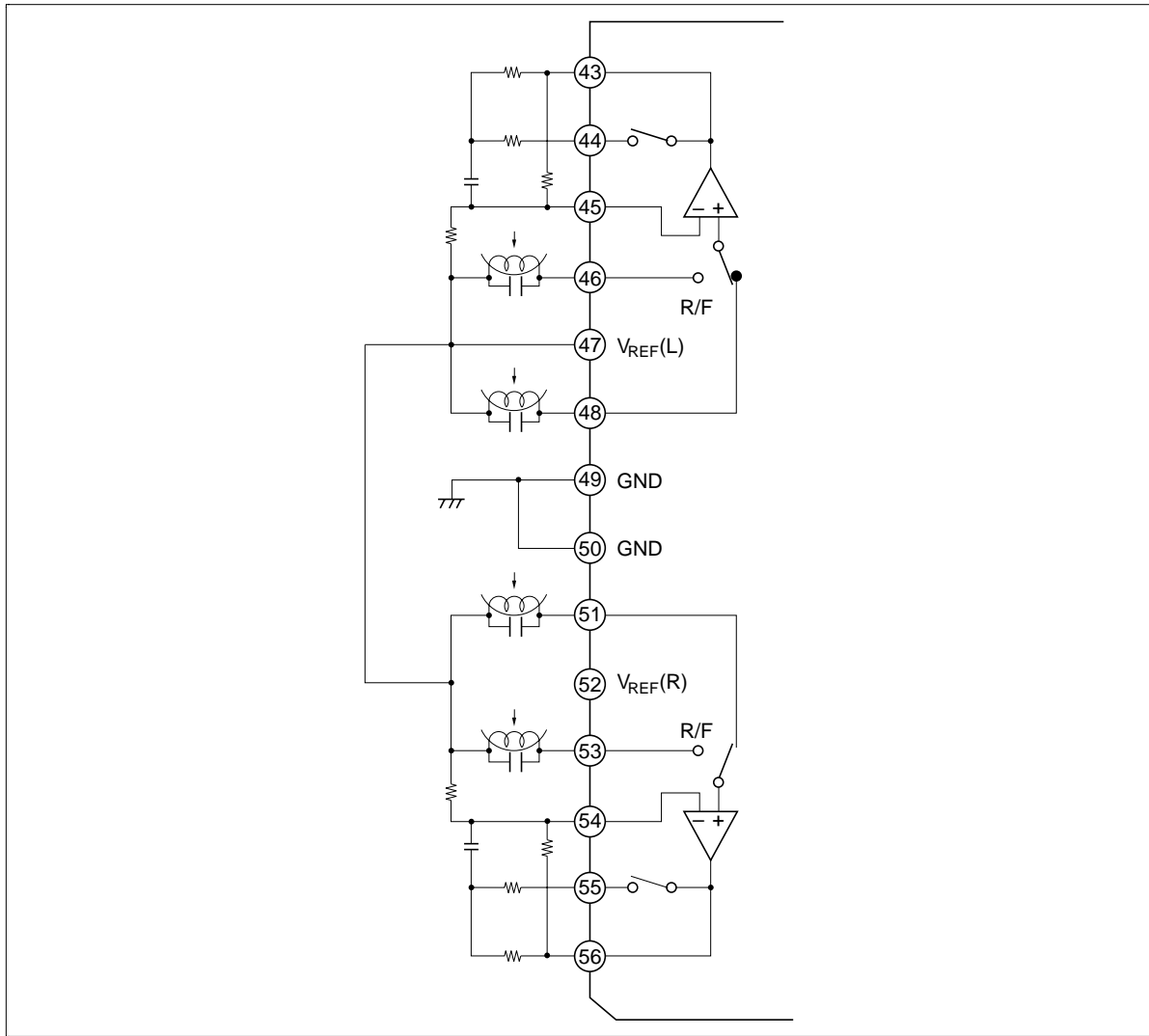
Figure 3 Application Circuit
