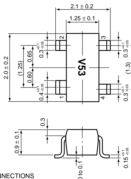
PACKAGE OUTLINE 18
