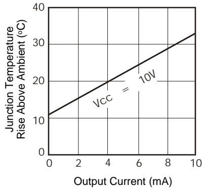
JUNCTION TEMP. RISE VS. OUTPUT CURRENT
