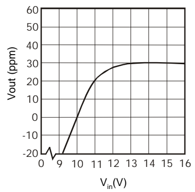
CHANGE IN OUTPUT VOLTAGE VS. INPUT VOLTAGE
