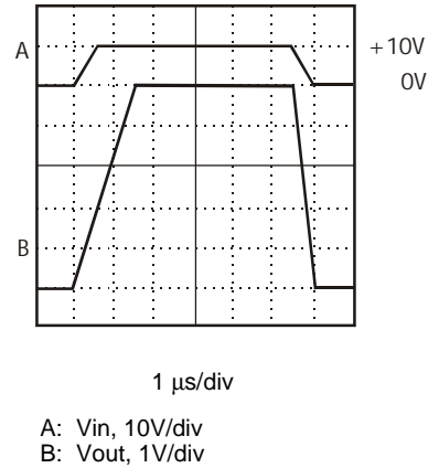
TURN-ON AND TURN-OFF TRANSIENT RESPONSE
