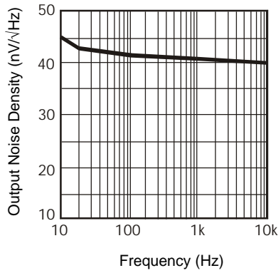
OUTPUT NOISE-VOLTAGE DENSITY vs. FREQUENCY
