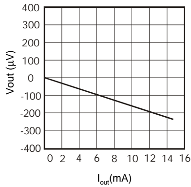
CHANGE IN OUTPUT VOLTAGE VS. OUTPUT CURRENT
