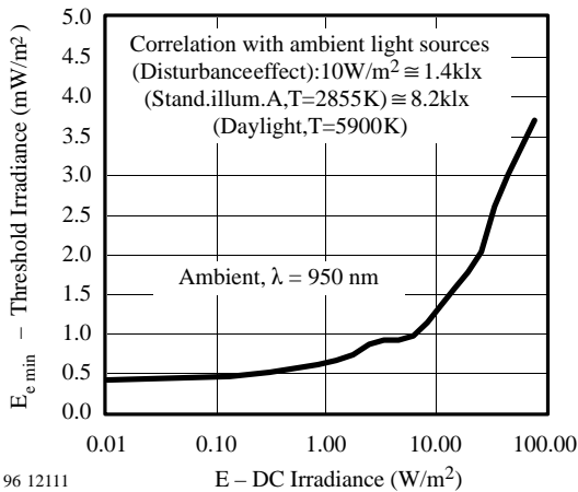
96 12111 Figure 3. Sensitivity in Bright Ambient
