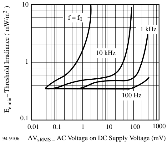
94 9106 Figure 5. Sensitivity vs. Supply Voltage Disturbances
