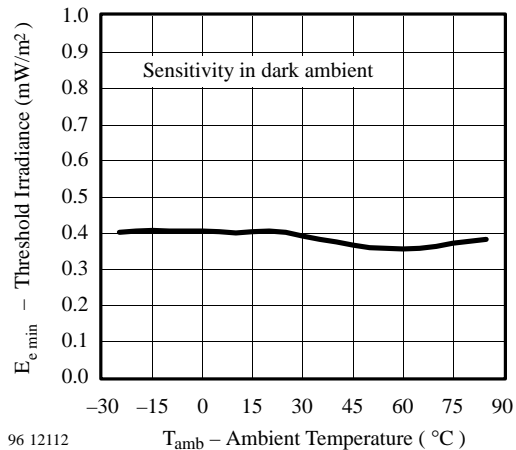
96 12112 Figure 6. Sensitivity vs. Ambient Temperature
