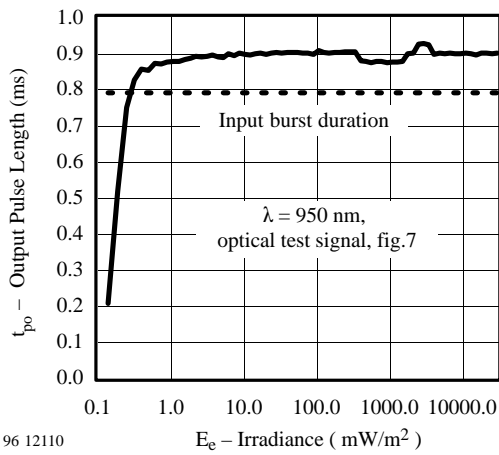
96 12110 Figure 2. Sensitivity in Dark Ambient
