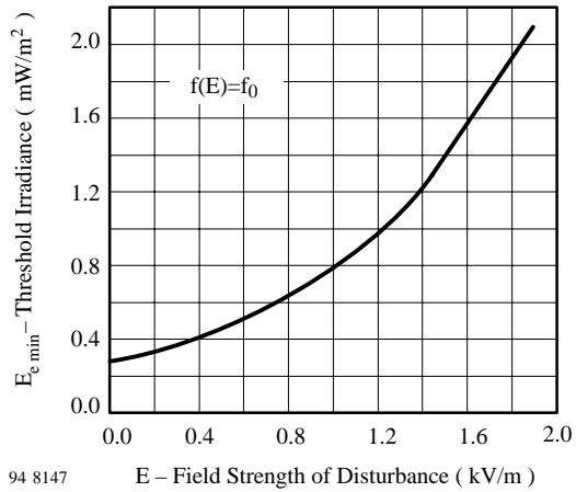
94 8147 Figure 4. Sensitivity vs. Electric Field Disturbances
