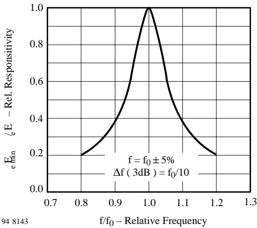
94 8143 Figure 1. Frequency Dependence of Responsivity
