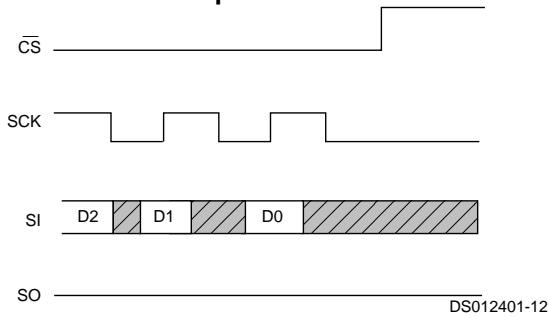
FIGURE 10. Write Sequence
