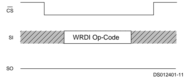
FIGURE 9. Write Disable
