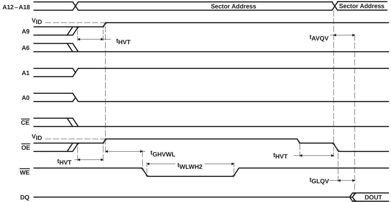
Figure 21. AC Waveform for Sector-Protect Operation
