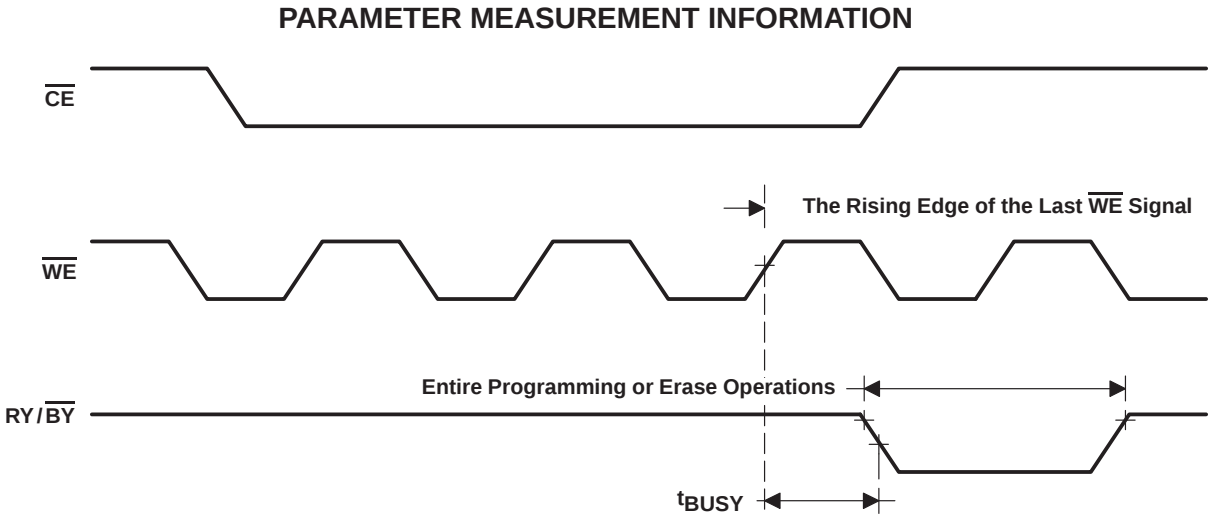
Figure 28. RY/ \overline{BY} Timing Diagram During Program/Erase Operations
