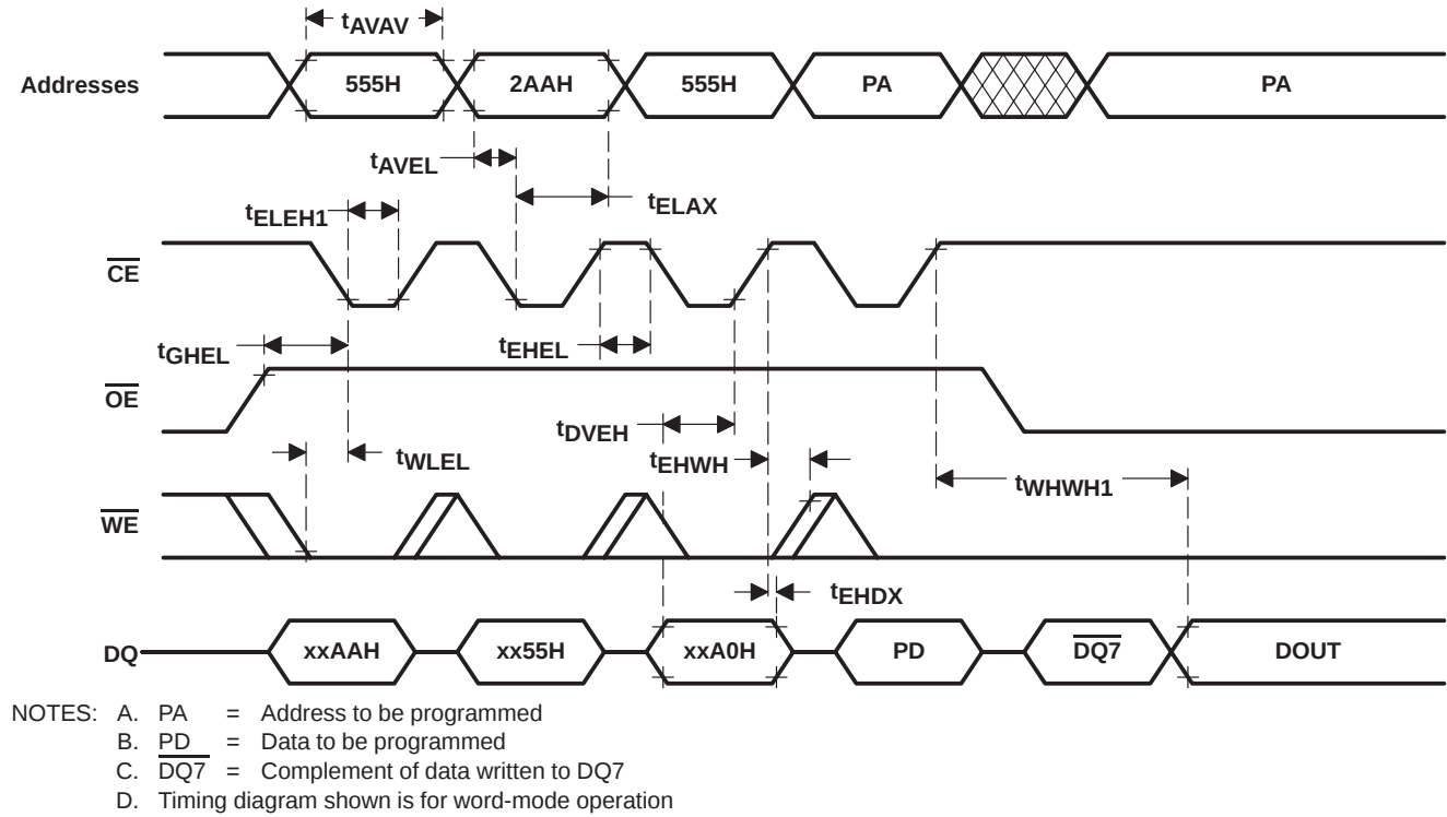
Figure 11. Alternate \overline{CE} -Controlled Write Operation
