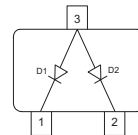
BAT17-06 BAT17-06W
