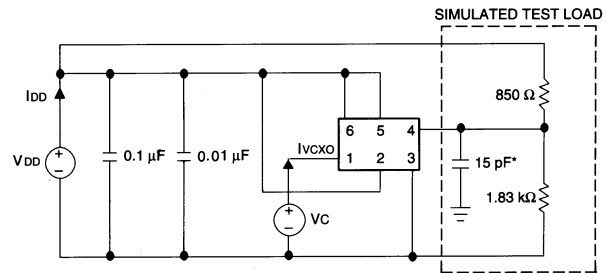
Figure 2. Output Test Conditions ( T_{amb} = 25 \pm 5^\circ\text{C} )
