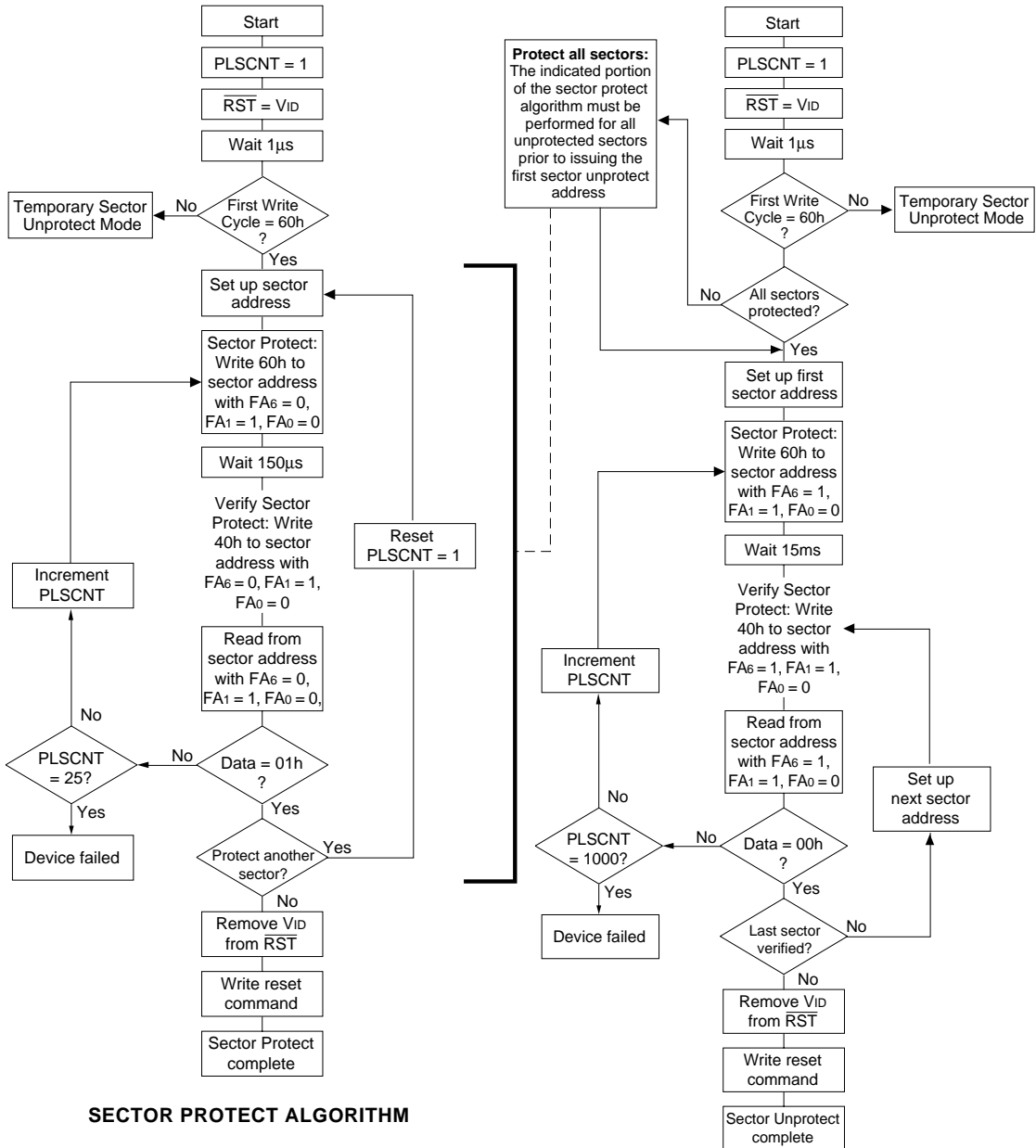
FIG. 5 SECTOR PROTECT/UNPROTECT ALGORITHMS
