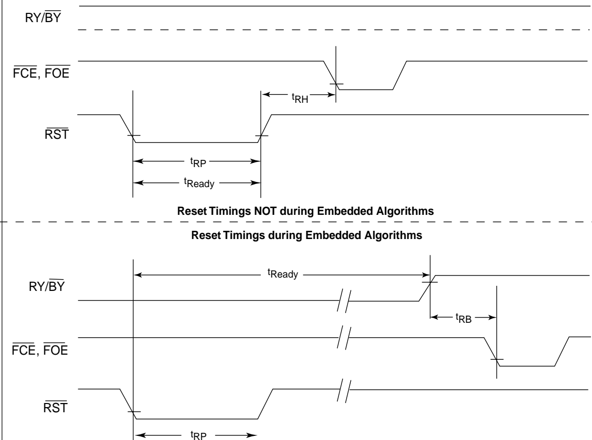
FIG. 19 HARDWARE RESET ( \overline{\text{RST}} )
