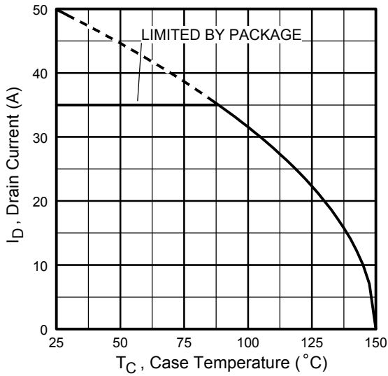
Case Temperature
