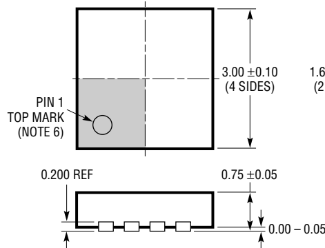
DD Package 8-Lead Plastic DFN (3mm \times 3mm) (Reference LTC DWG # 05-08-1698)
