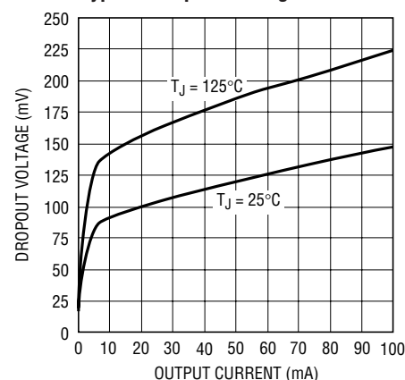
Typical Dropout Voltage
