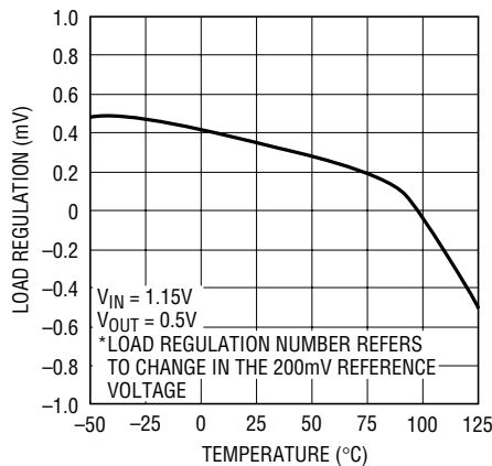
Load Regulation \Delta I_L = 1\text{mA to }100\text{mA}
