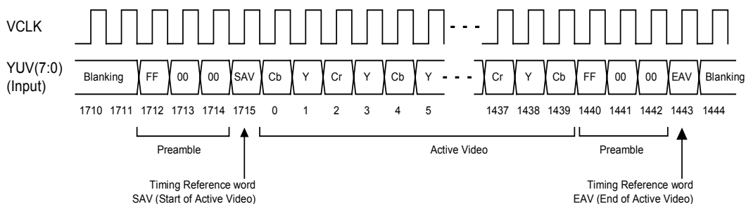
Figure 11. ITU-R BT656 Input
