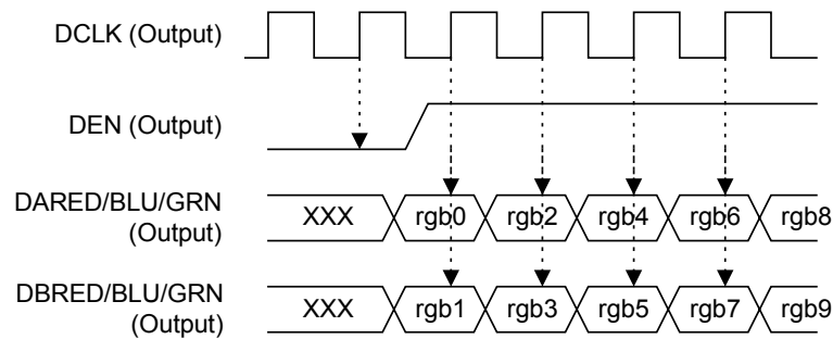
Figure 19. Double Pixel Wide Display Data
