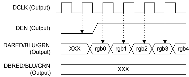
Figure 18. Single Pixel Width Display Data
