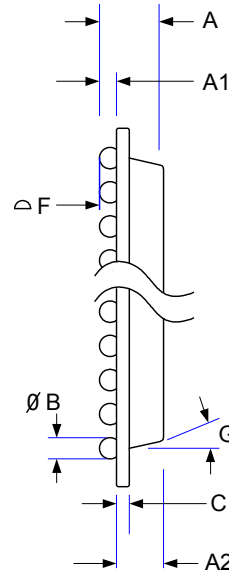
Figure 32. gm5060 292-pin Thermally Enhanced PBGA
