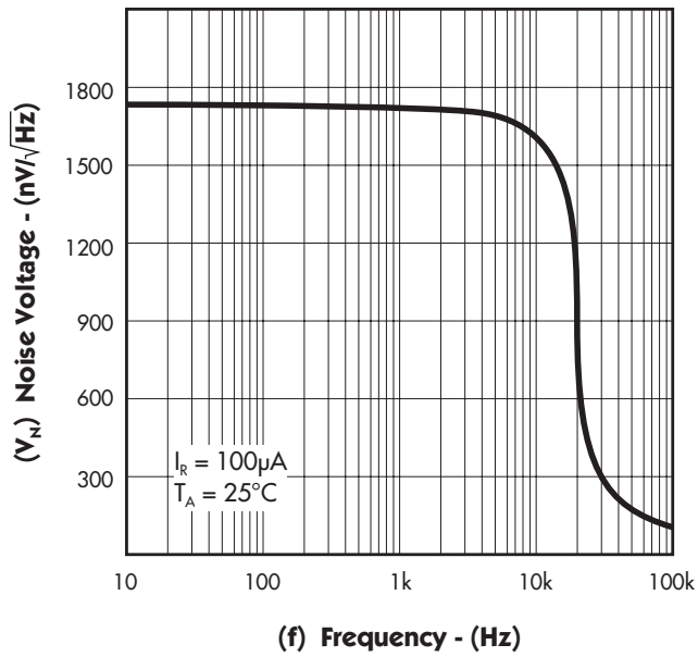
FIGURE 12. — NOISE VOLTAGE
