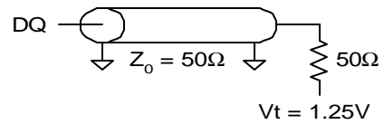
Fig. 3 OUTPUT LOAD EQUIVALENT
