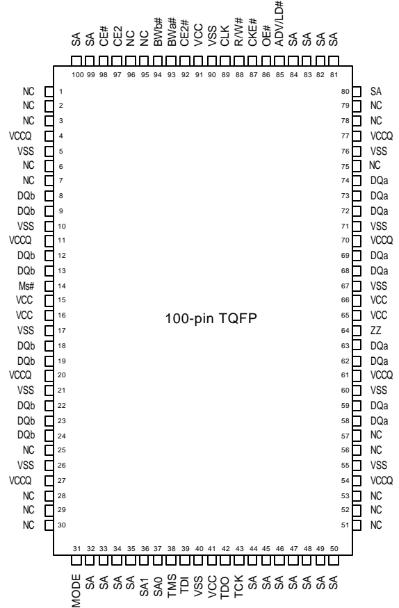
1Mx18, 100-PIN TQFP (Top View)
