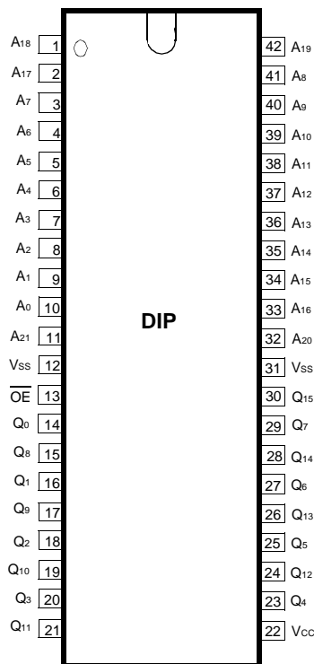
KM23C64000B
