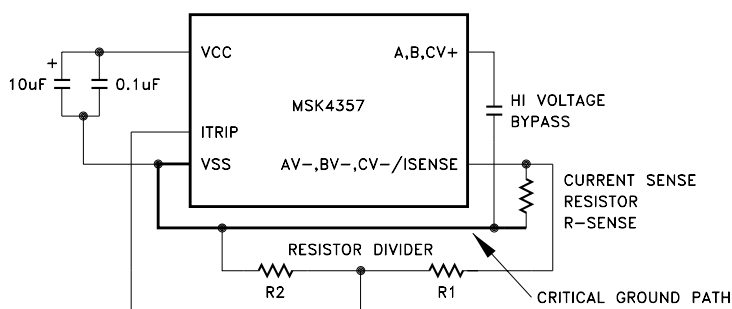
FIGURE 1 GROUNDING, BYPASSING, CURRENT SENSE
