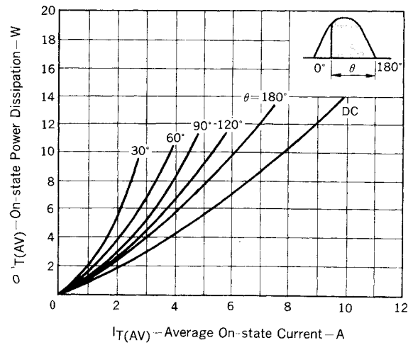
Fig. 10 P_{T(AV)} - I_{T(AV)} CHARACTERISTIC
