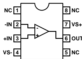
EL2160 (8-PIN PDIP, SO) TOP VIEW
