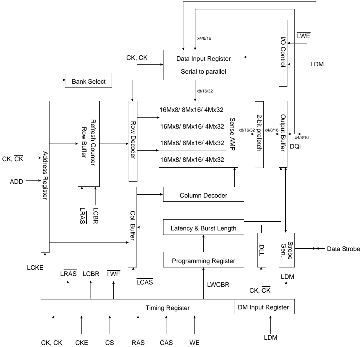
Block Diagram (32Mbit x 4 / 16Mbit x 8 / 8Mbit x 16 I/O x 4 Banks)
