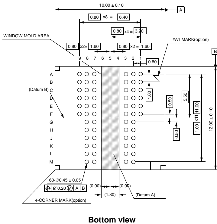
60Ball FBGA 512Mb Package Dimension
