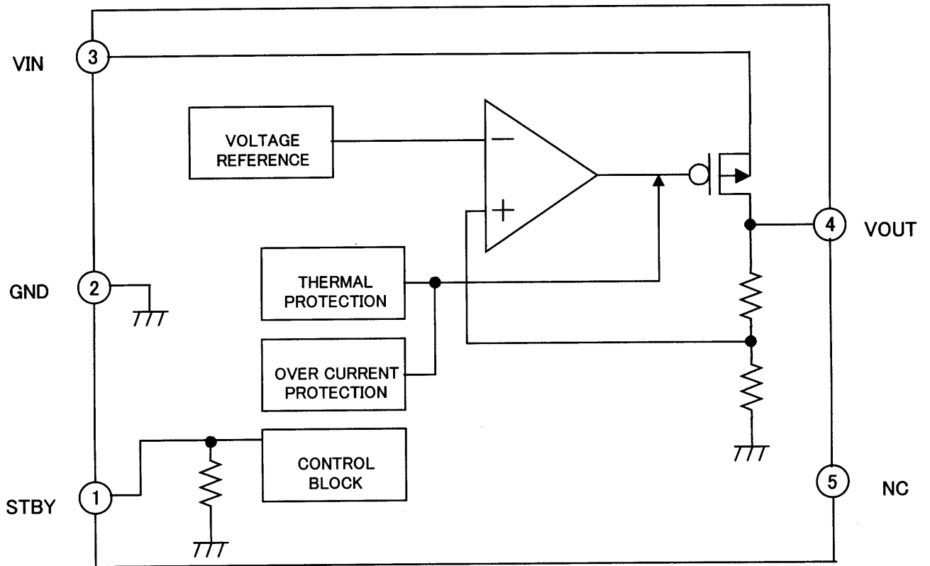
Fig.2 BLOCK DIAGRAM
