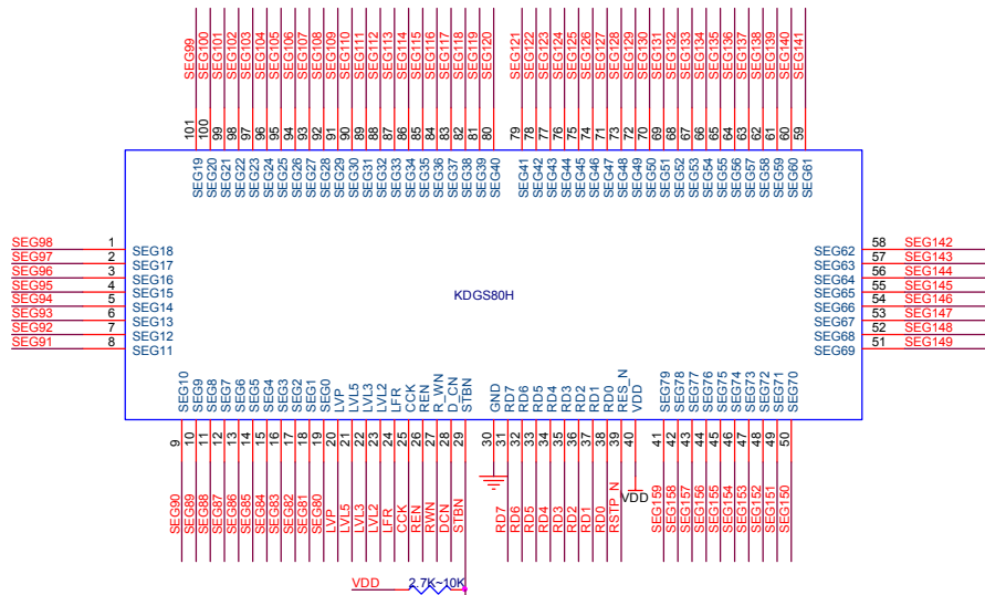
This application assumes 48COM X 80SEG configuration, and 80 SEG Extender KDG80H.
