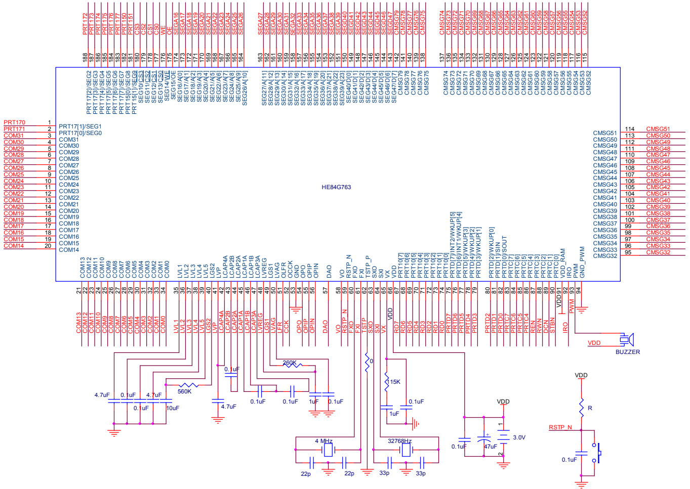
This application assumes 48COM X 80SEG configuration, and 80 SEG Extender KDG80H.
