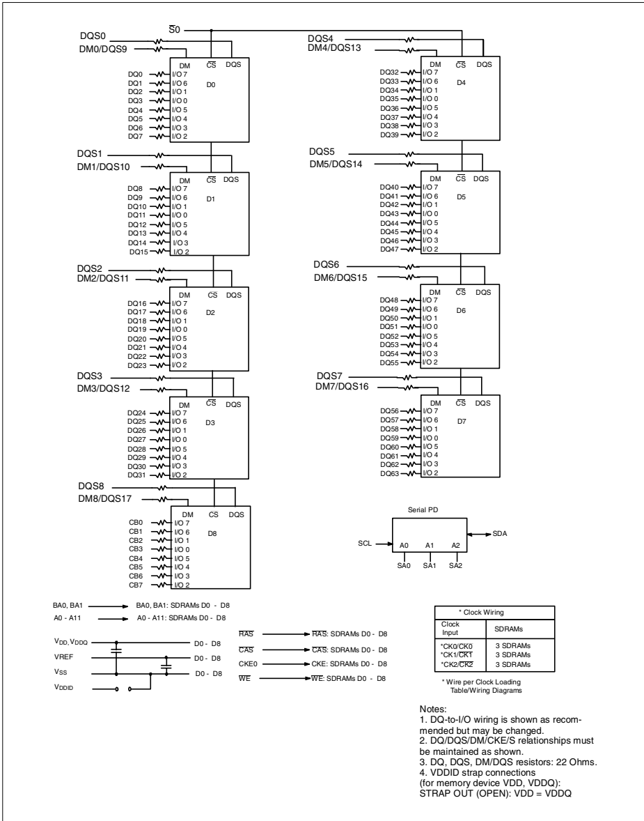
Block Diagram: One Bank 16M x 72 DDR-I SDRAM DIMM Module HYS72D16000GU using x8 organized SDRAMs
