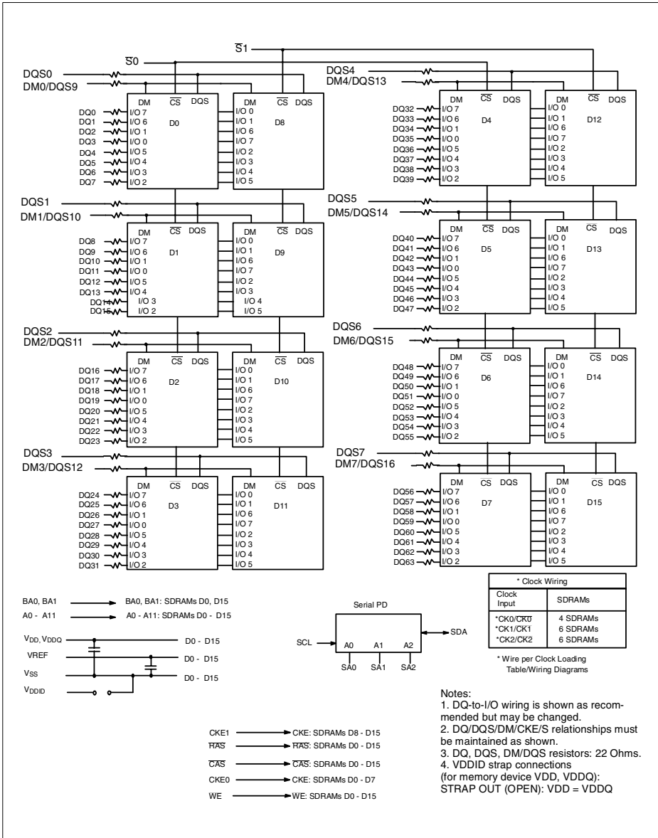
Block Diagram: Two Bank 32M x 64 DDR-I SDRAM DIMM Modules HYS64D32020GU using x8 Organized SDRAMs
