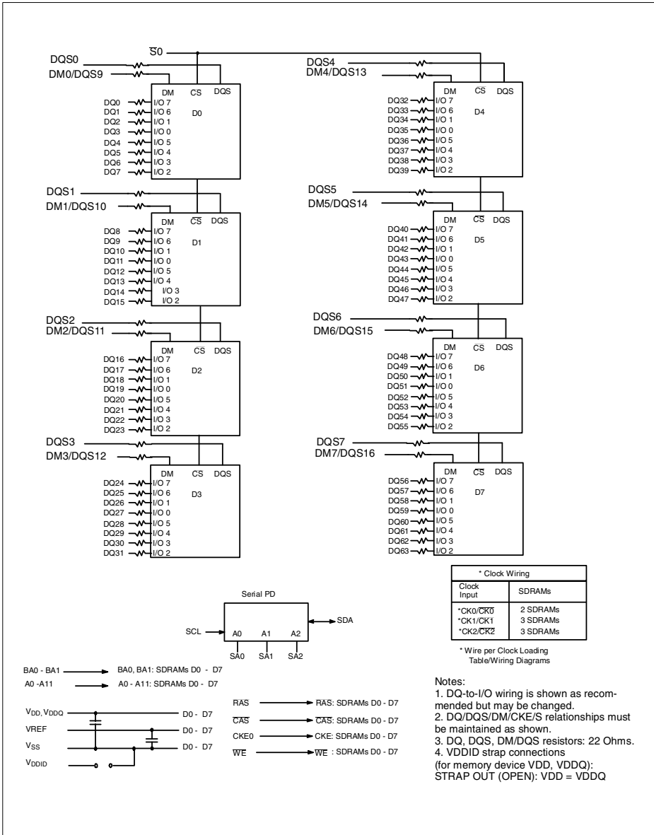
Block Diagram: One Bank 16M x 64 DDR-I SDRAM DIMM Module HYS64D16000GU using x8 organized SDRAMs
