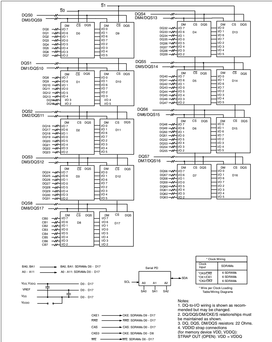
Block Diagram: Two Bank 32M x 72 DDR-I SDRAM DIMM Modules HYS72D32020GU using x8 Organized SDRAMs
