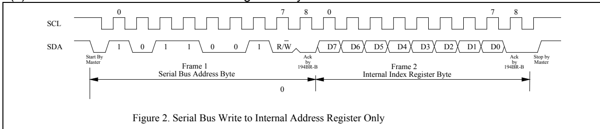
(b) Serial bus write to internal address register only
