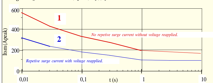
Fig.3 Surge current : I_{t\text{sm}}(\text{Apeak}) = f(t) for 50A models with I_{t\text{sm}} = 550\text{A}
