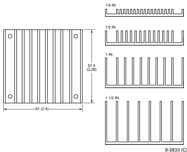
Figure 44. Transverse Heat Sink
