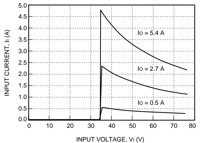
Figure 4. Typical JW150R Input Characteristics at Room Temperature
