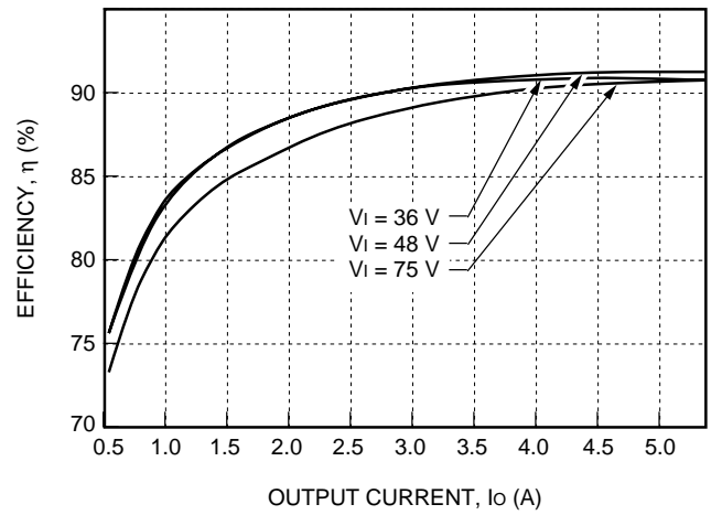
Figure 12. Typical JW150R Converter Efficiency vs. Output Current at Room Temperature
