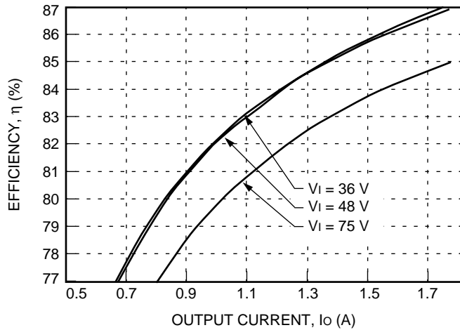
Figure 9. Typical JW050R Converter Efficiency vs. Output Current at Room Temperature
