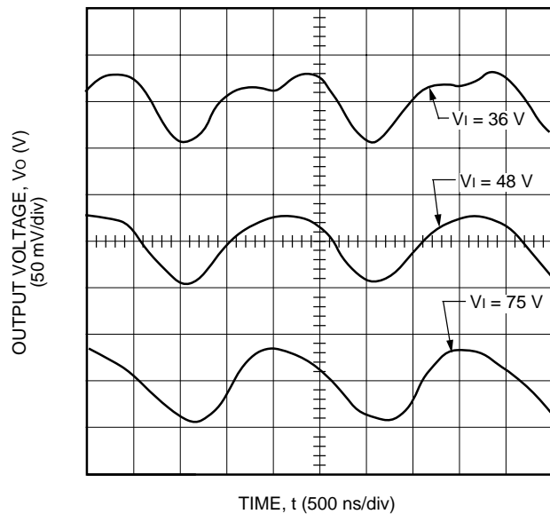
Figure 16. Typical JW150R Output Ripple Voltage at Room Temperature, 36 Vdc to 75 V Input, and 5.4 A Output
