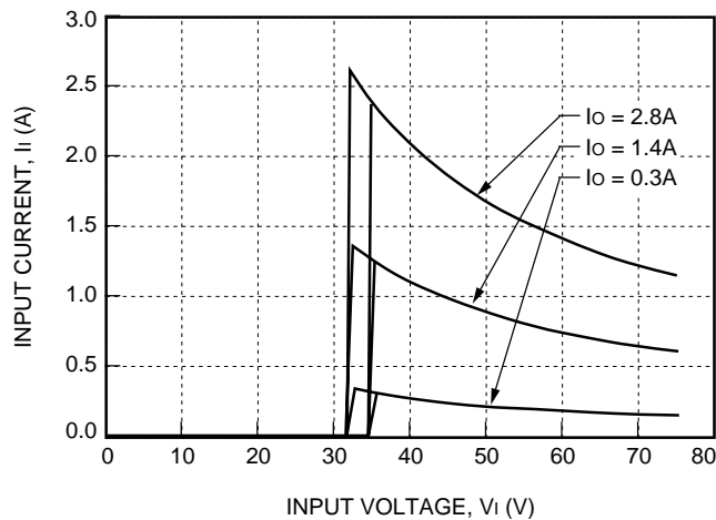
Figure 2. Typical JW075R Input Characteristics at Room Temperature
