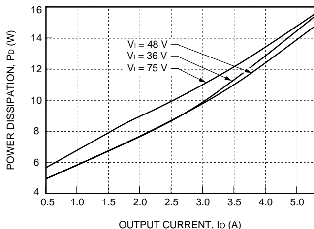
Figure 40. JW150R Power Dissipation vs. Output Current at 25 °C
