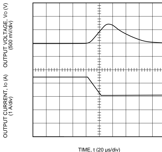
Figure 19. Typical JW100R Transient Response to Step Decrease in Load from 50% to 25% of Full Load at Room Temperature and 48 Vdc Input (Waveform Averaged to Eliminate Ripple Component.)
