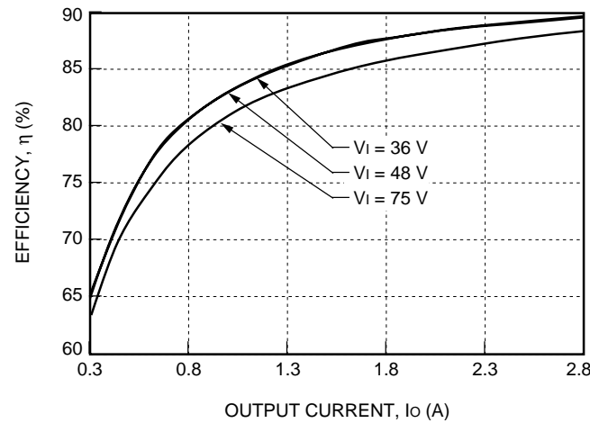
Figure 10. Typical JW075R Converter Efficiency vs. Output Current at Room Temperature
