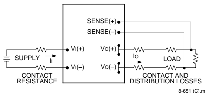
Figure 30. Effective Circuit Configuration for Single-Module Remote-Sense Operation
