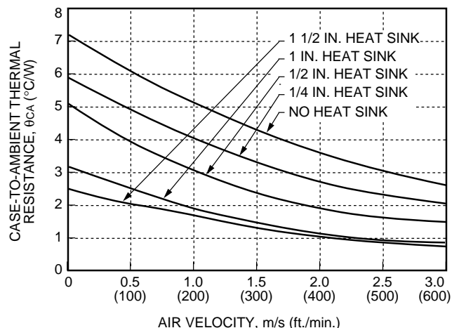
Figure 41. Case-to-Ambient Thermal Resistance Curves; Either Orientation
