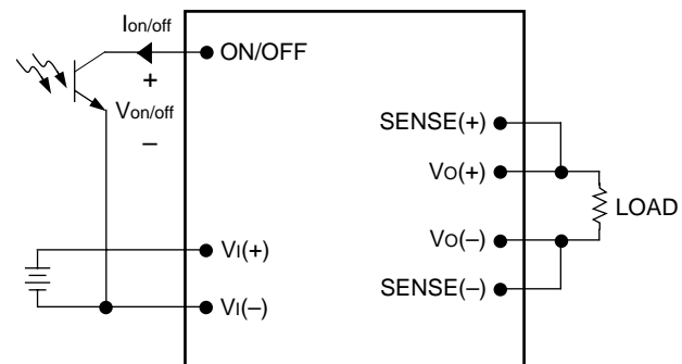
Figure 29. Remote On/Off Implementation
