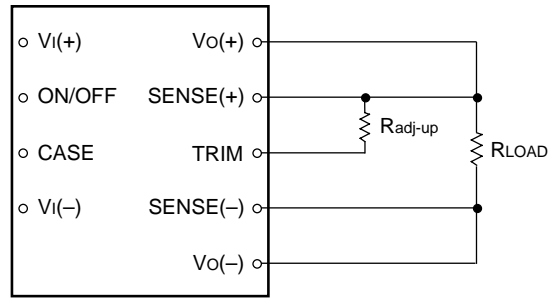
Figure 33. Circuit Configuration to Increase Output Voltage
