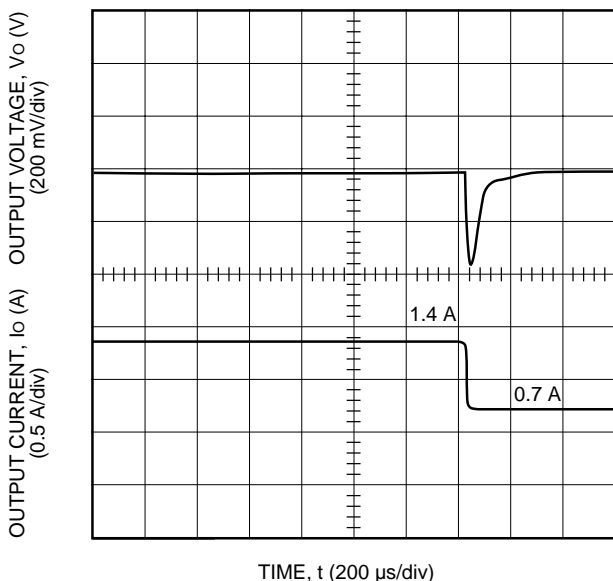
Figure 17. Typical JW050R Transient Response to Step Decrease in Load from 50% to 25% of Full Load at Room Temperature and 48 Vdc Input (Waveform Averaged to Eliminate Ripple Component.)
