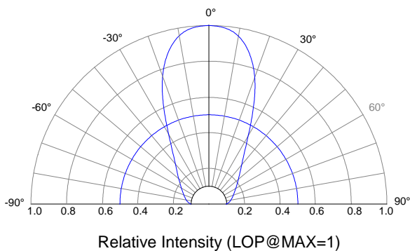
Beam Pattern
