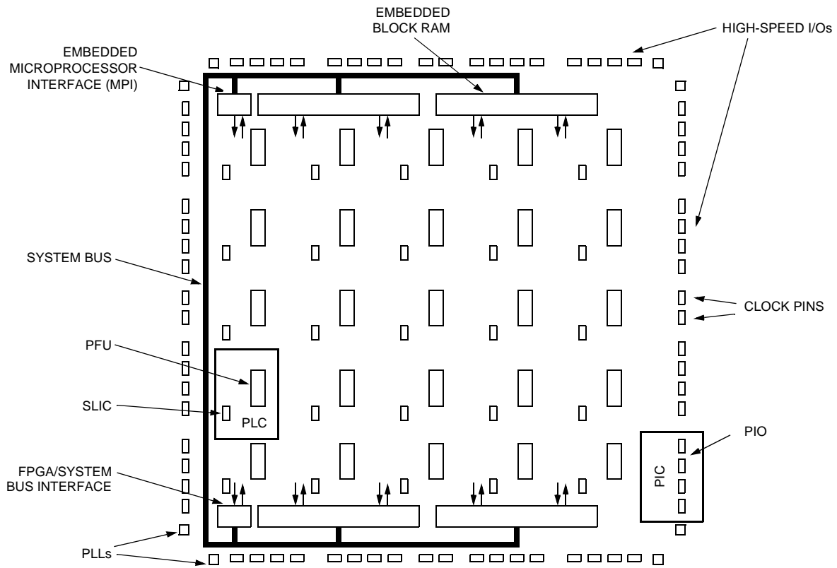
Figure 1. Series 4 FPGA Block Diagram
