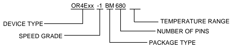
Figure 2. OR4Exx, -1 Speed Grade, 680-pin Plastic Ball Grid Array Multilayer (PBGAM)
