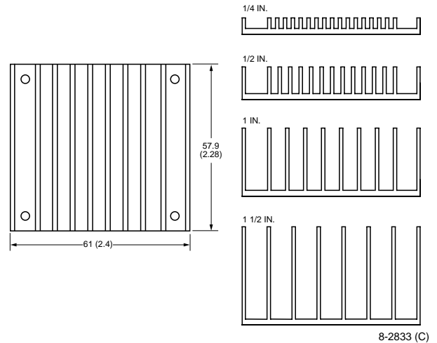
Figure 36. Transverse Heat Sink
