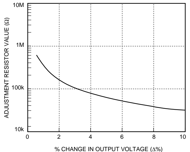
Figure 25. Resistor Selection for Increased Output Voltage
