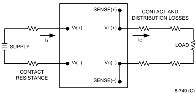
Figure 18. Peak-to-Peak Output Noise Measurement Test Setup
