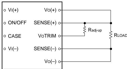
Figure 24. Circuit Configuration to Increase Output Voltage
