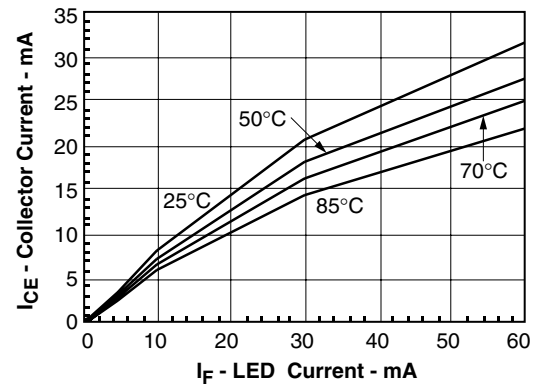
Figure 6. Collector-emitter current versus temperature and LED current
