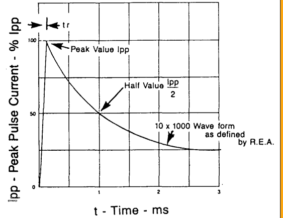
FIGURE 2 Pulse Waveform Test waveform parameters: t_r=10 \mu s , t_p=1000 \mu s
