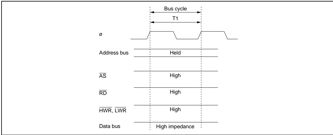
Pin States during On-Chip Memory Access
