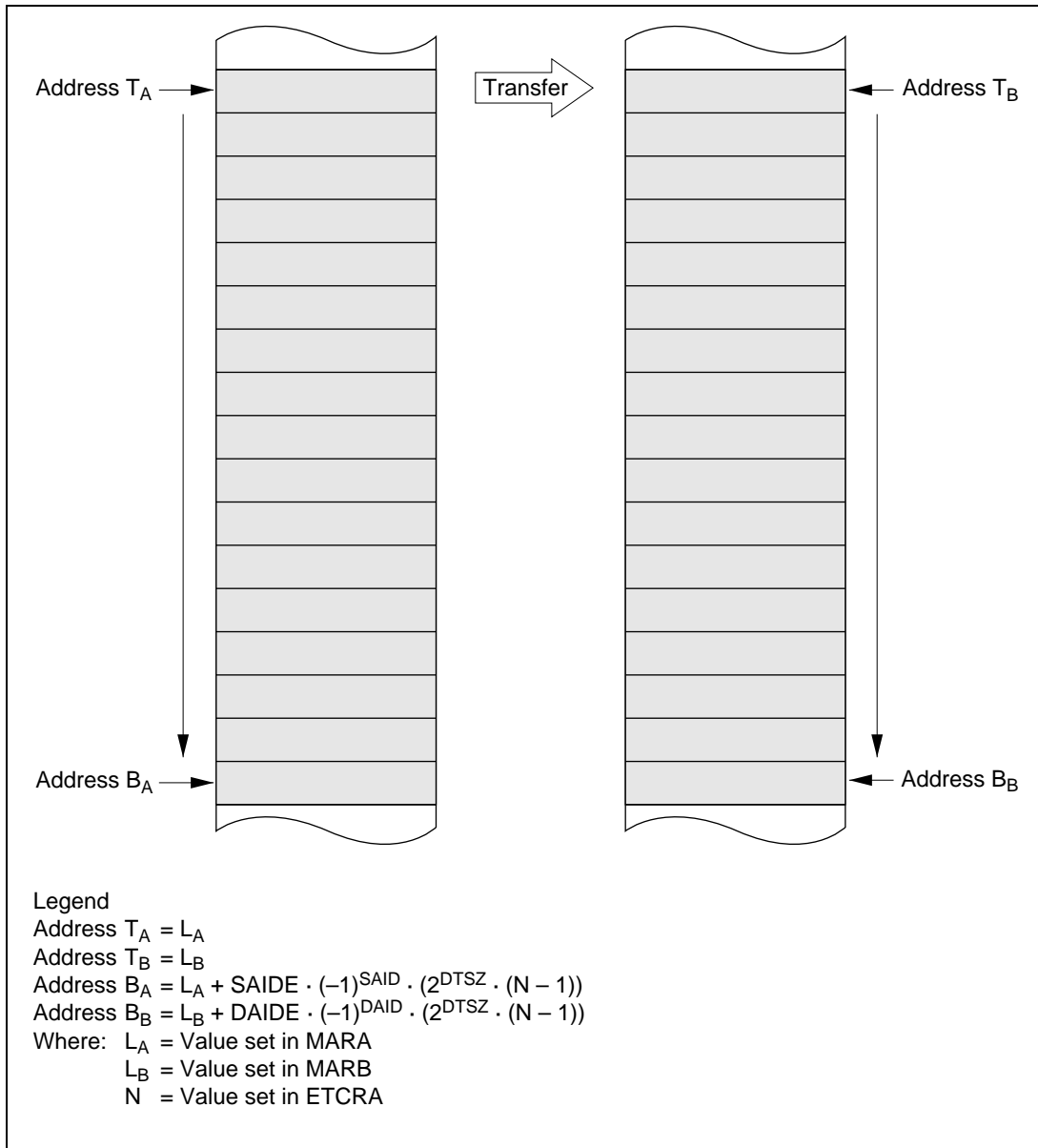
Operation in Normal Mode
