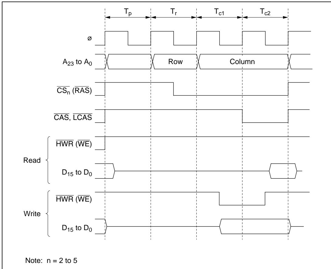
Example of 2-CAS Type DRAM Connection
