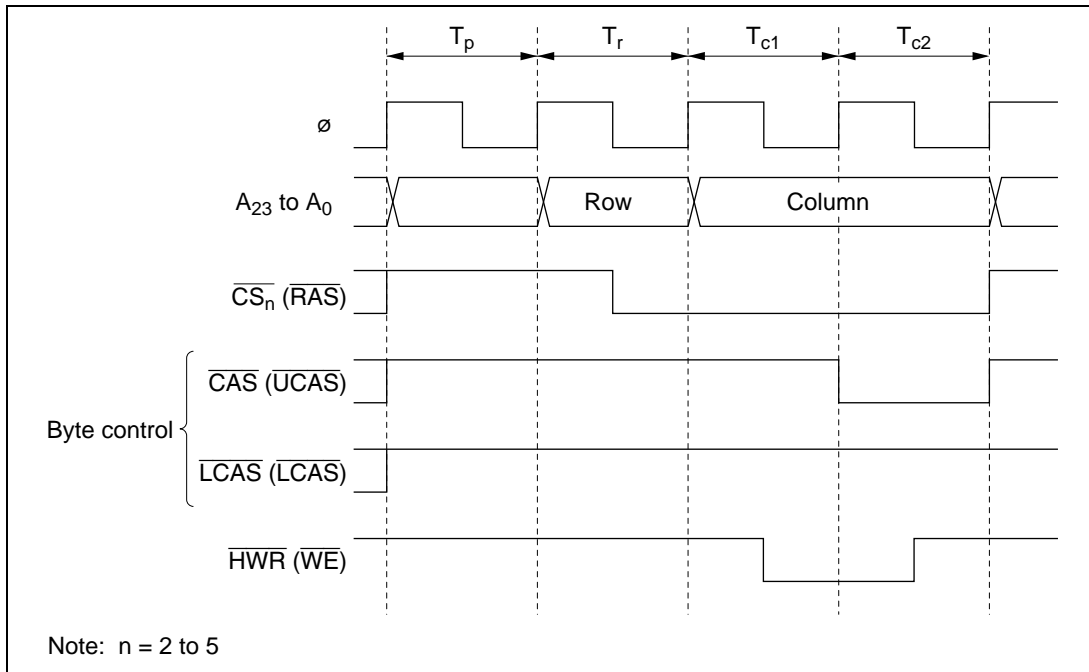
Byte Access Control Timing (Upper Byte Write Access)
