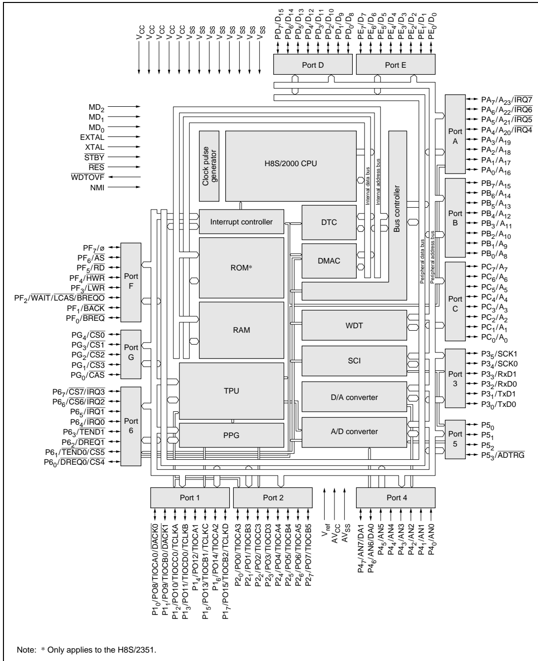
Block Diagram
