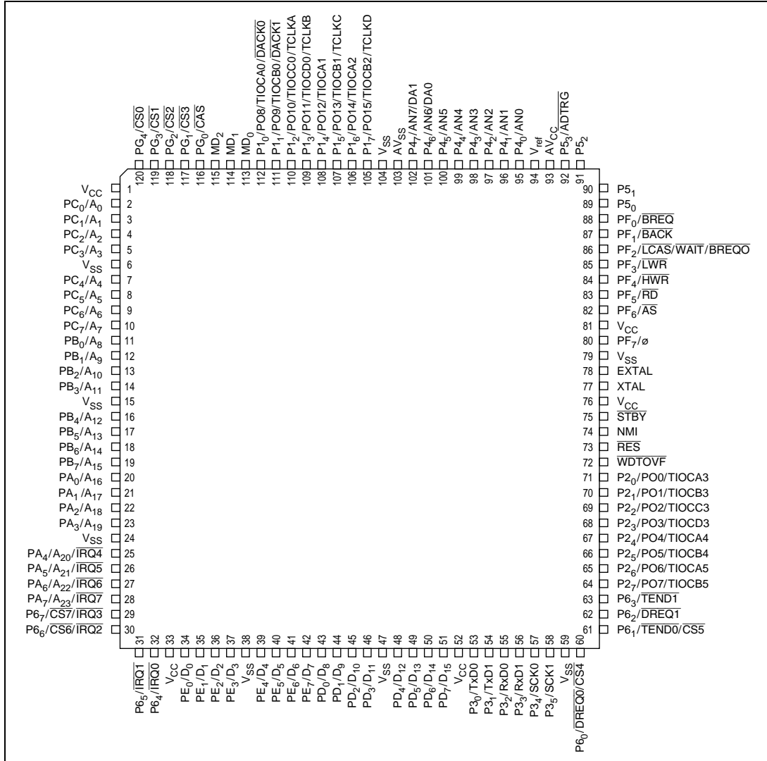
120-Pin Plastic TQFP (TFP-120: Top View)
