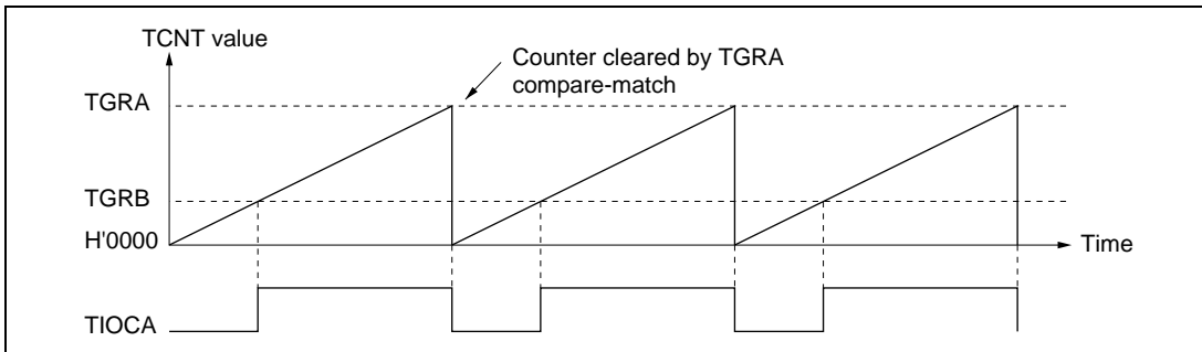
Operation in PWM Mode 1
