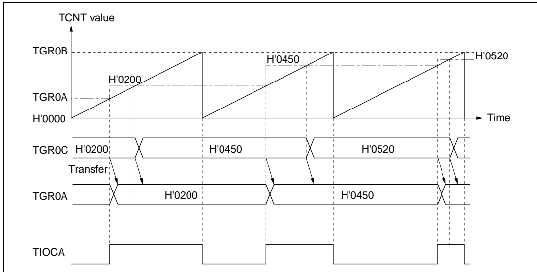
Example of Buffer Operation (1) (When TGR Is an Output Compare Register)
