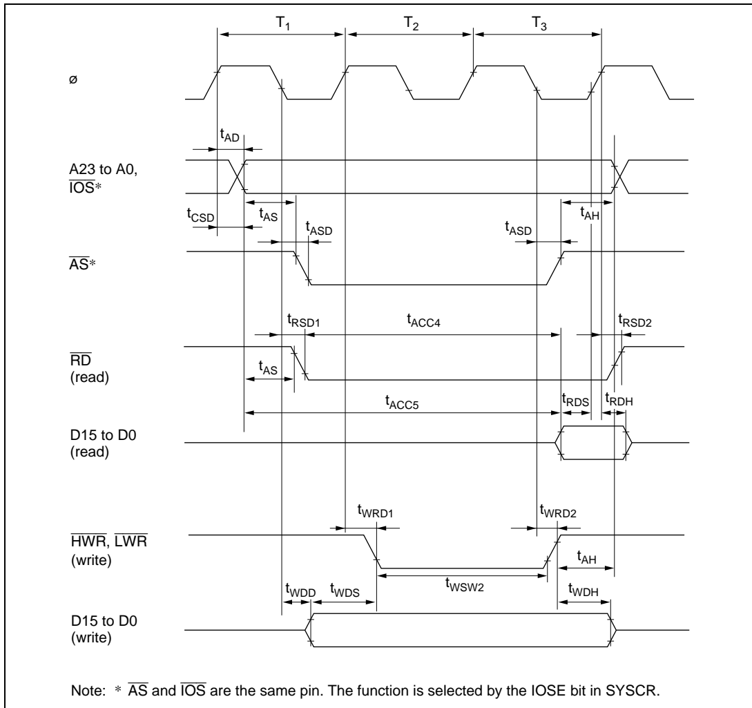
Figure 25.10 Basic Bus Timing (Three-State Access)
