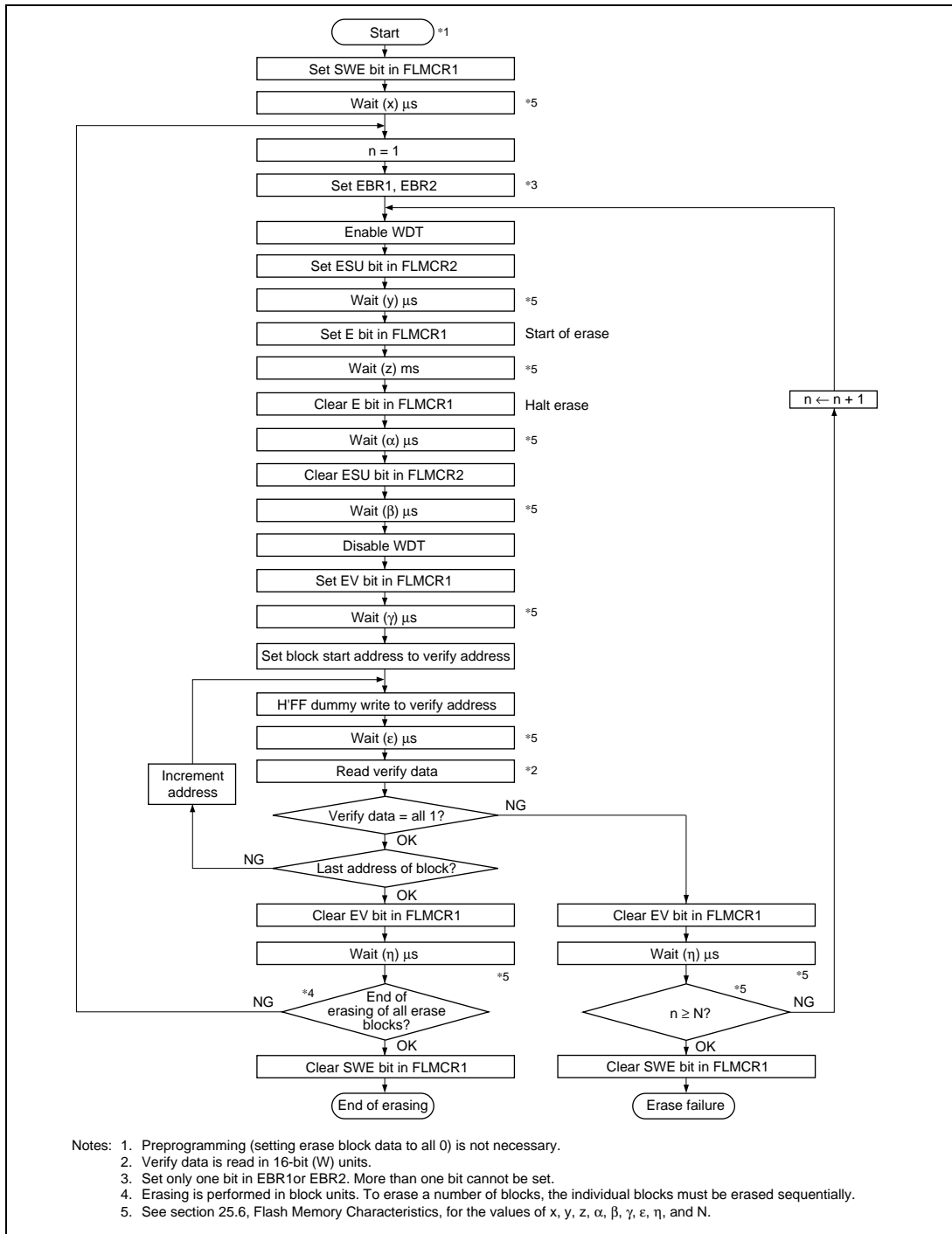
Figure 22.13 Erase/Erase-Verify Flowchart (Single-Block Erase)
