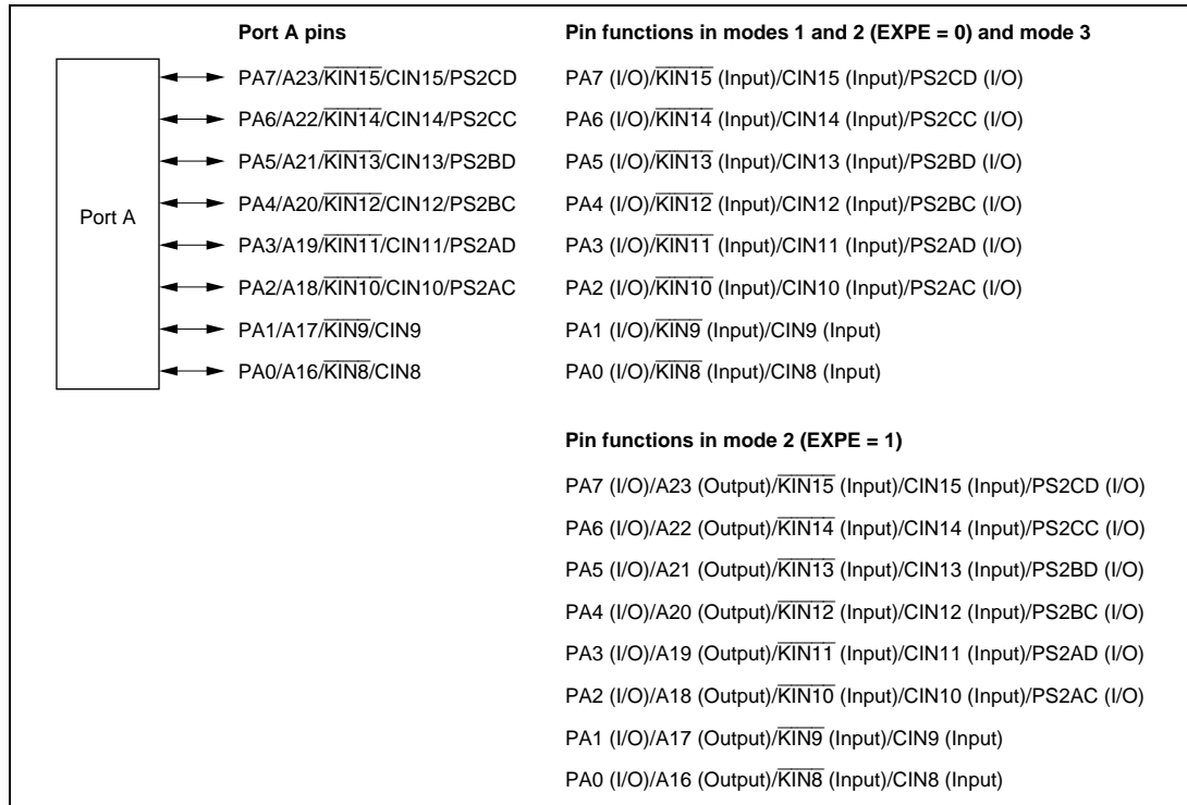
Figure 8.18 Port A Pin Functions
