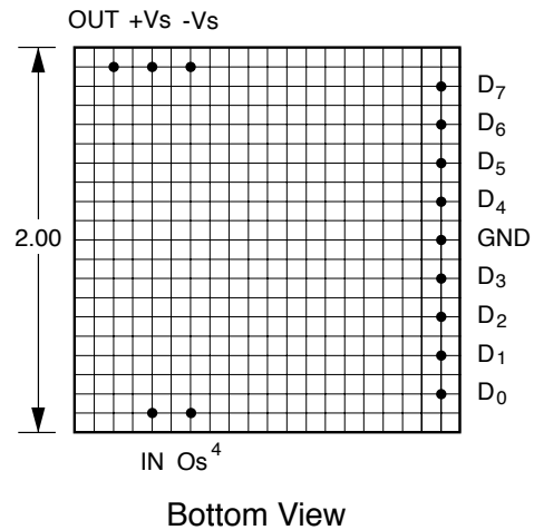
Filter Mounting Assembly-See FMA-02A
